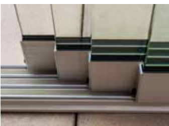
Floor frame
